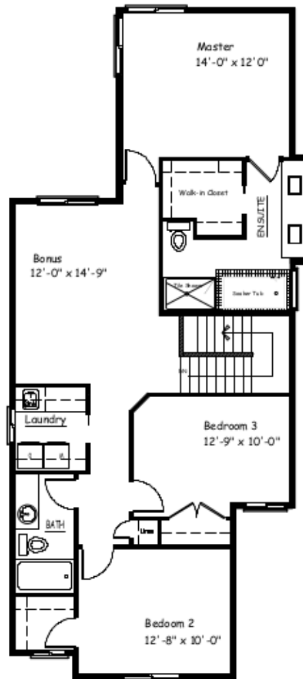
Upper Floor 1140 sq. ft.
