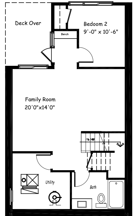
Walk-Out Basement Dev. Option
