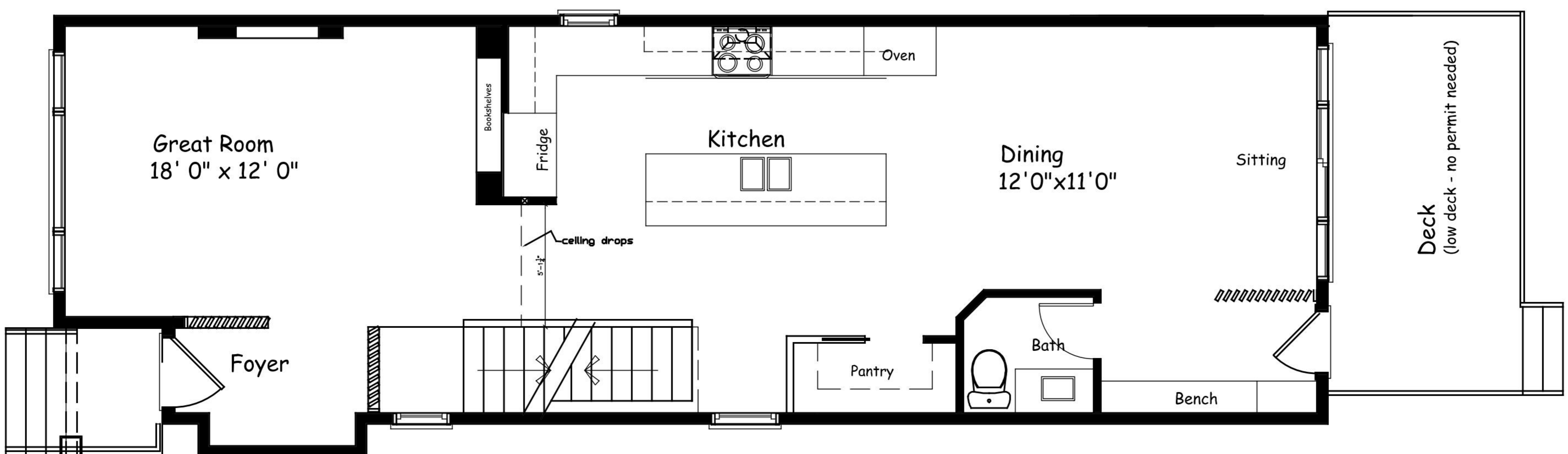
Main Floor 893 sq.ft. 2063 Total sq.ft.
