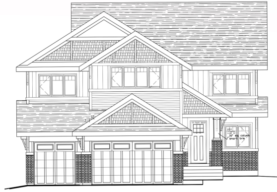
Front Elevation - Craftsman
